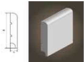
LAGRUS CLASSIC R10 80 x 16
